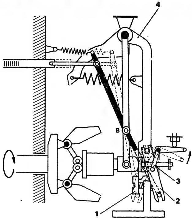
Fig. 11 Normal service operation
